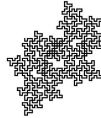
Lion Curve
