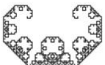
Lévy Curve
