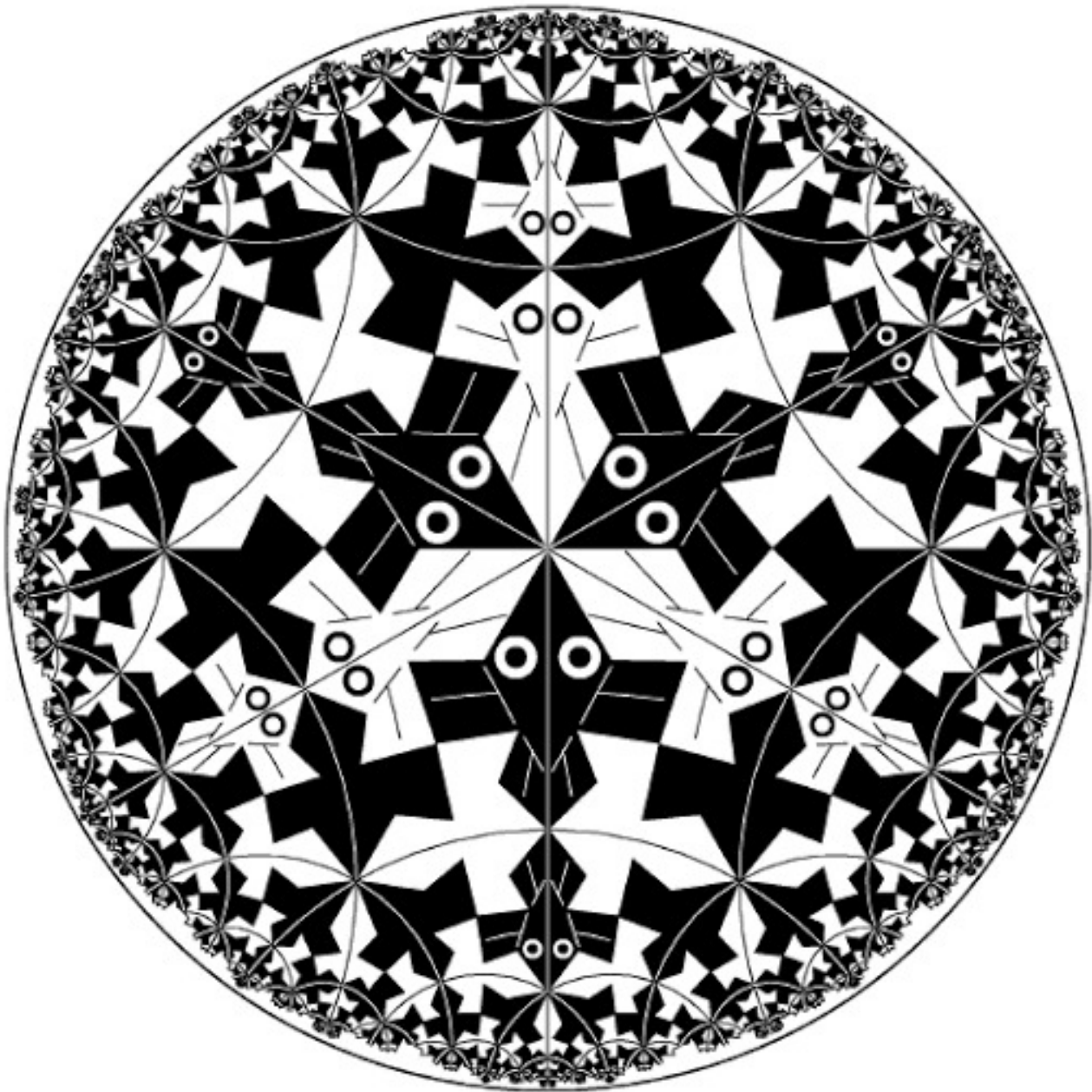
FIGURE 7. Circle Limit I, by M. C. Escher. What kind of orbifold is shown here?
