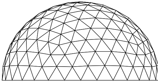
Figure 1: 6V Geodesic Dome and Buckminster Fuller Stamp
