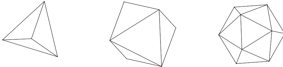
Figure 2: Platonic Solids
