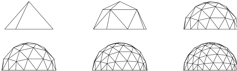
Figure 10: 1V through 6V Octahedral Domes
